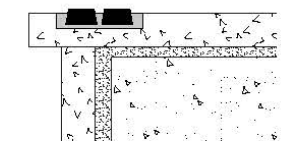
Terrazzo/Marble Tread rabbeted into tread
